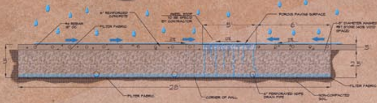
2 PERMEABLE PAVEMENT SECTION VIEW "OIL BROKEN DOWN BY NATURAL MICROBES, WITHIN 18\"/>
